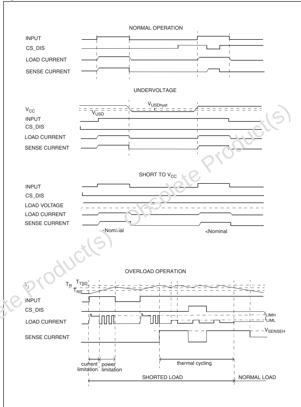
Figure 35. Waveforms
