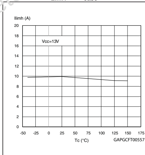
Figure 16. I_{LIMH} vs T_{case}
