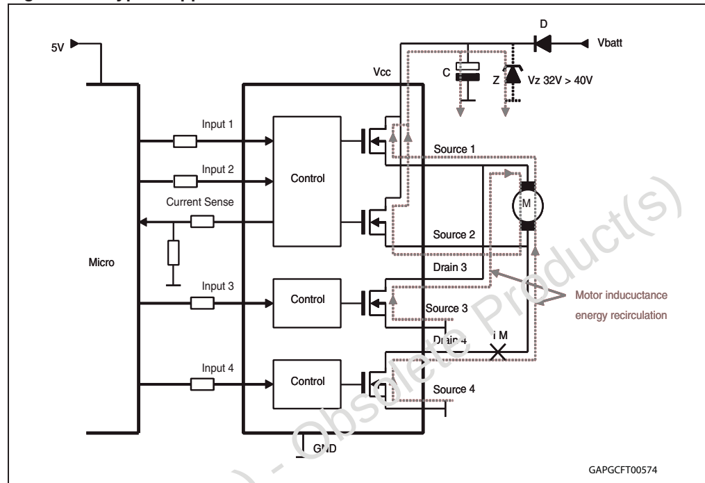
Figure 33. Typical application schematic
